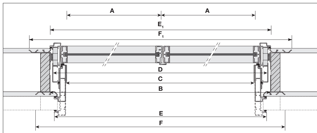
Porta doppia - stipite SMALL Double swing door - SMALL jamb Двойная дверь - Косяк SMALL
