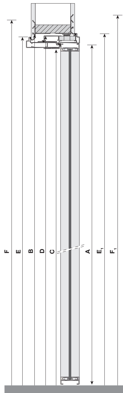
Porta doppia - stipite SMALL Double swing door - SMALL jamb Двойная дверь - Косяк SMALL
